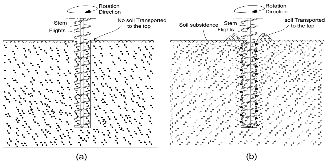
Fig. (1) (a) Ideal conditions, flights full of soil, (b) Over-flying
