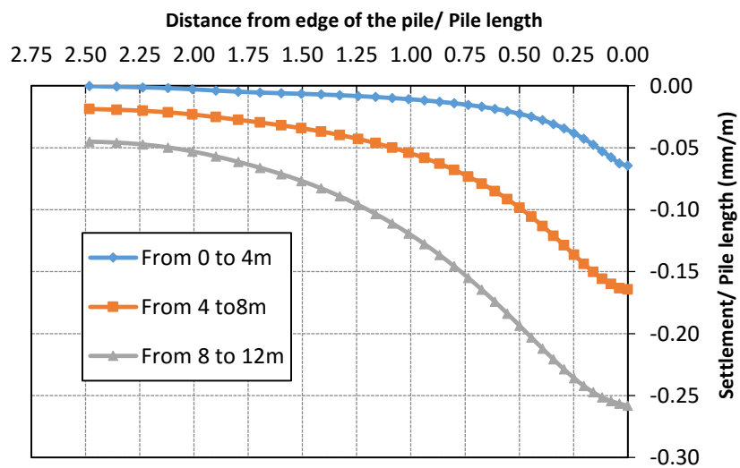
Fig. (6) Settlement induced due to lateral stress decrease in the first three segments
