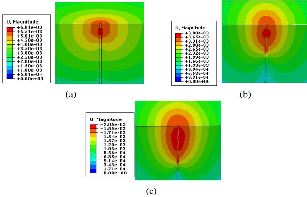
Fig. (7) Settlement contour calculated due to loss of lateral support at three segments, (a) segment 1, (b) segment 2, and (c) segment 3
