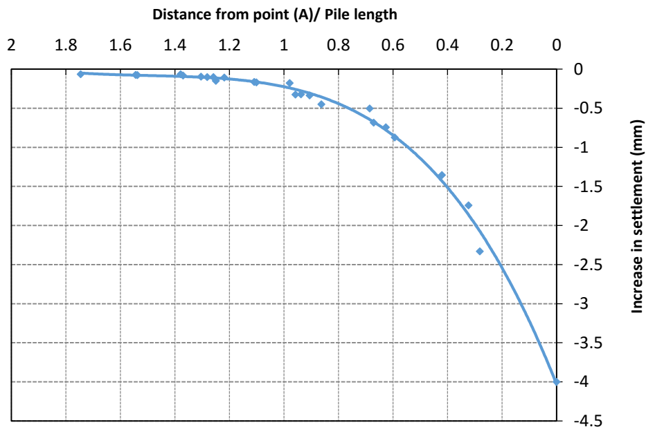
Fig. (9) Increase in settlement happened due to over-flighting during CFA piles drilling with distance
