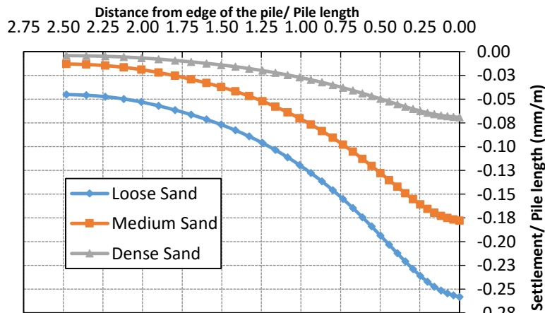
Fig. (8) Settlement calculated for unfavorable CFA pile drilling with change in sand relative density
